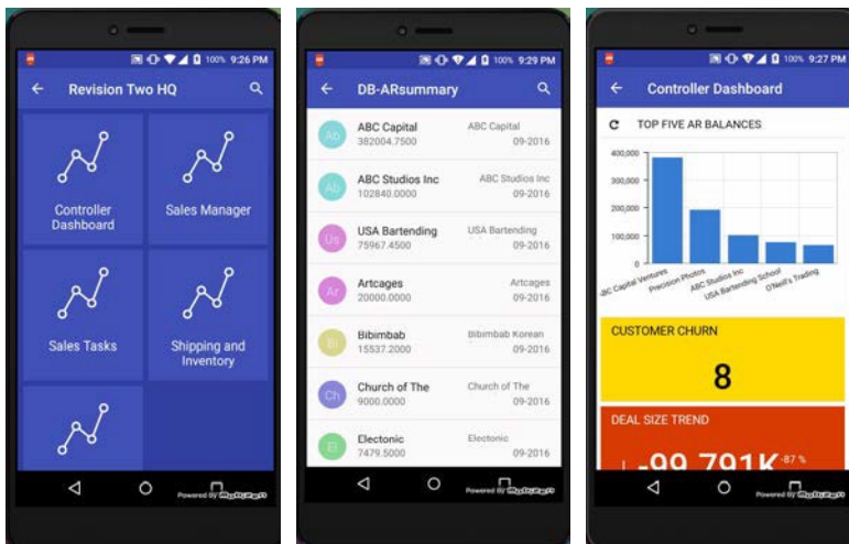
Dashboards
