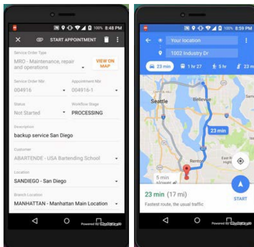
Map integration
